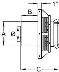
Low Restriction Horizontal Termination (LRHT)
